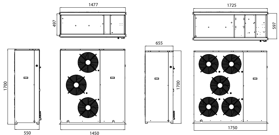
PBM 25
