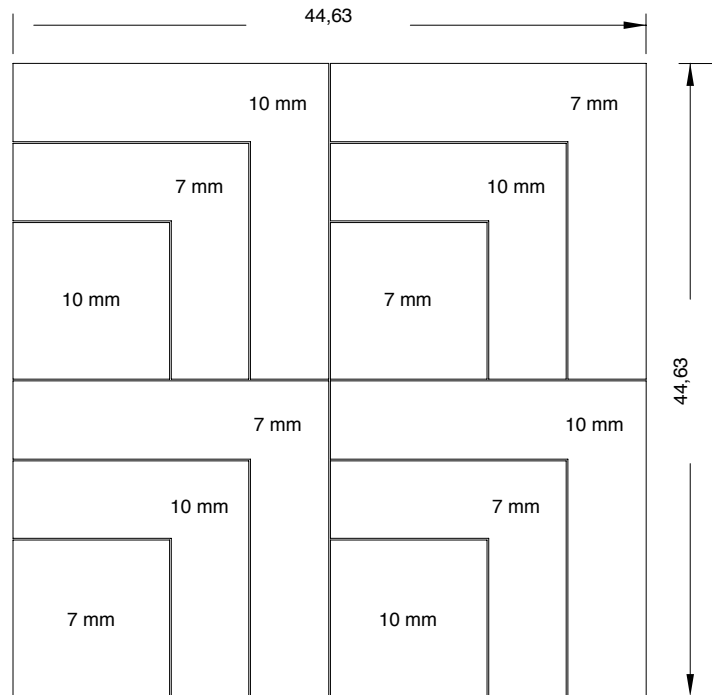
Nanoconcept 7.0 beige decor ramp (44,63 x 44,63 cm - 17.57" x 17.57")
