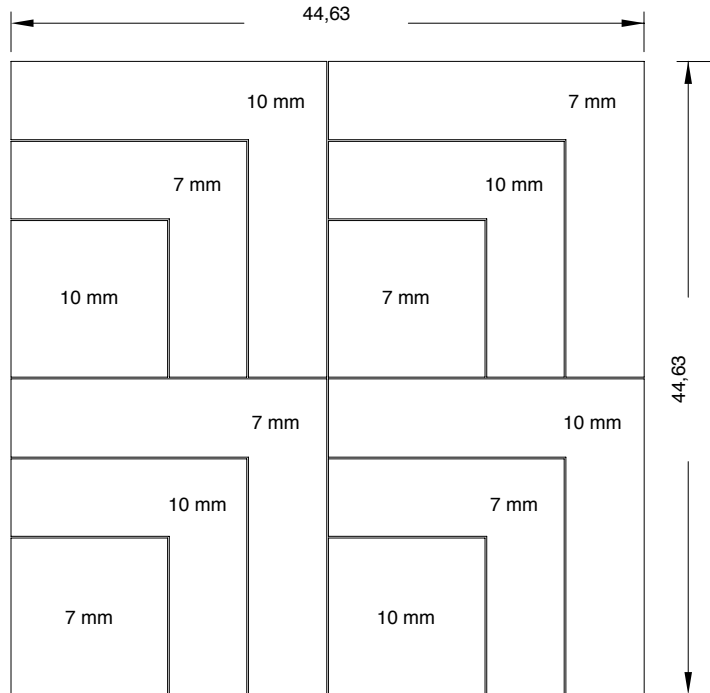
Nanoconcept 7.0 black decor ramp (44,63 x 44,63 cm - 17.57" x 17.57")
