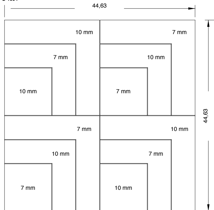
Nanoconcept 7.0 grey decor ramp (44,63 x 44,63 cm - 17.57" x 17.57")
