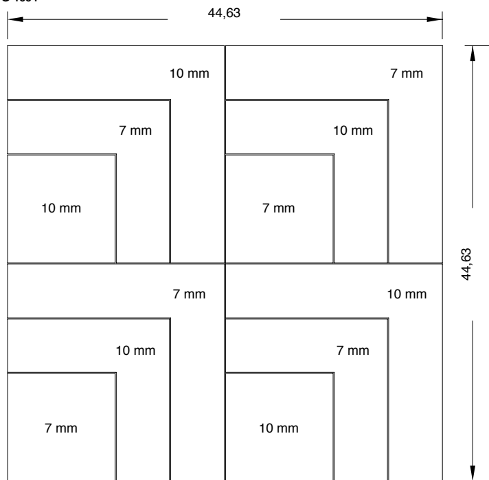
Nanoconcept 7.0 anthracite decor ramp (44,63 x 44,63 cm - 17.57" x 17.57")
